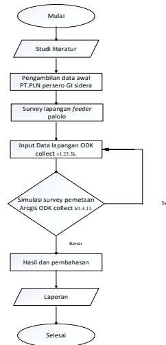
Gambar 3.1 Diagram flowcart
